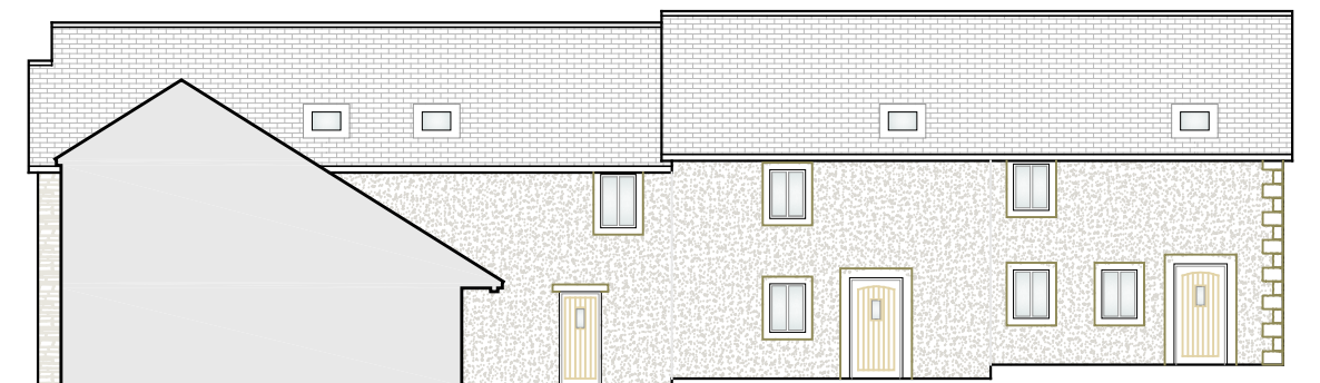
PROPOSED ELEVATION G-G
