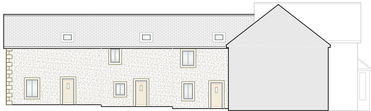
PROPOSED ELEVATION D-D
